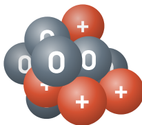
carbon-13
