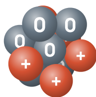
carbon-12
