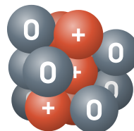
carbon-14
